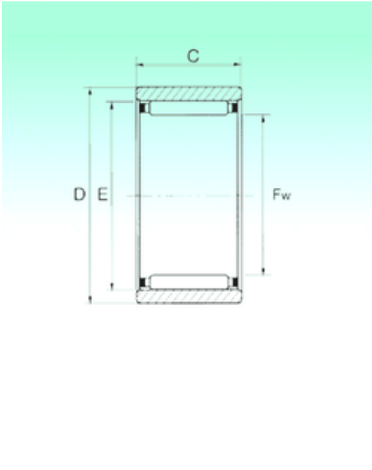
RNAO 70x90x30 Bearing 2D drawings and 3D CAD models
